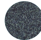
GRAPHITE SPECTRUM
